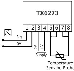
2 WIRE PROBE CONNECTIONS
